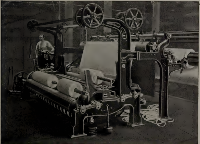
"M & W" Patented Four Drum Winder in operation.
